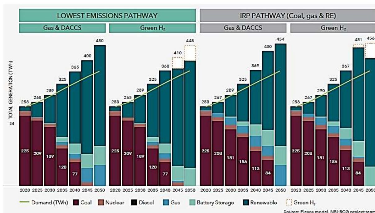
FIGURE 17: ELECTRICITY GENERATION BY SOURCE, LOWEST EMISSION PATHWAYS AND IRP PATHWAYS 112
