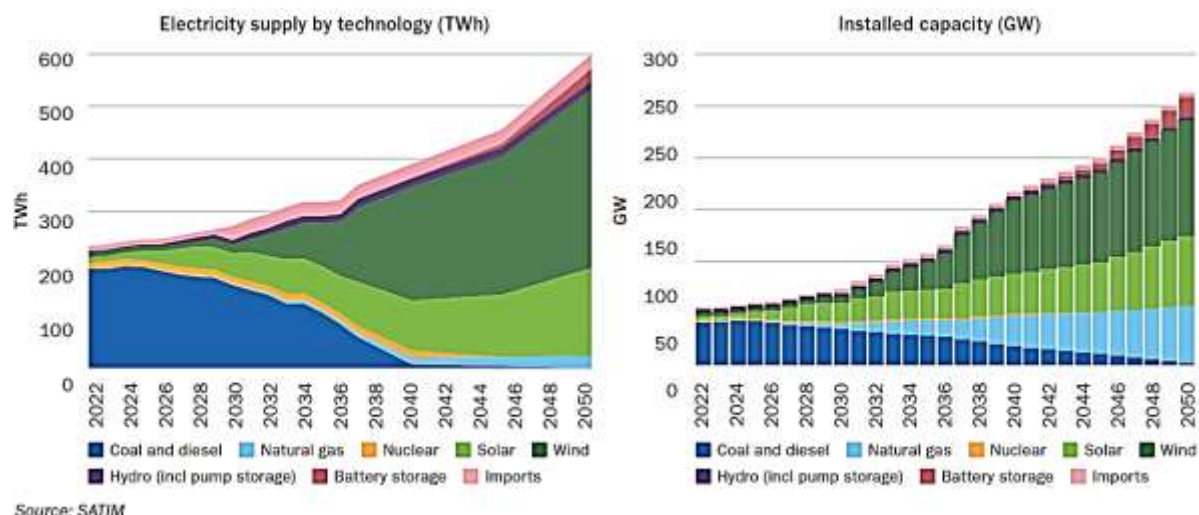
FIGURE 6: NET ZERO REFERENCE SCENARIO FOR THE ELECTRICITY SECTOR BY ELECTRICITY SUPPLY TECHNOLOGY (TWh) AND INSTALLED CAPACITY (GW) 70
