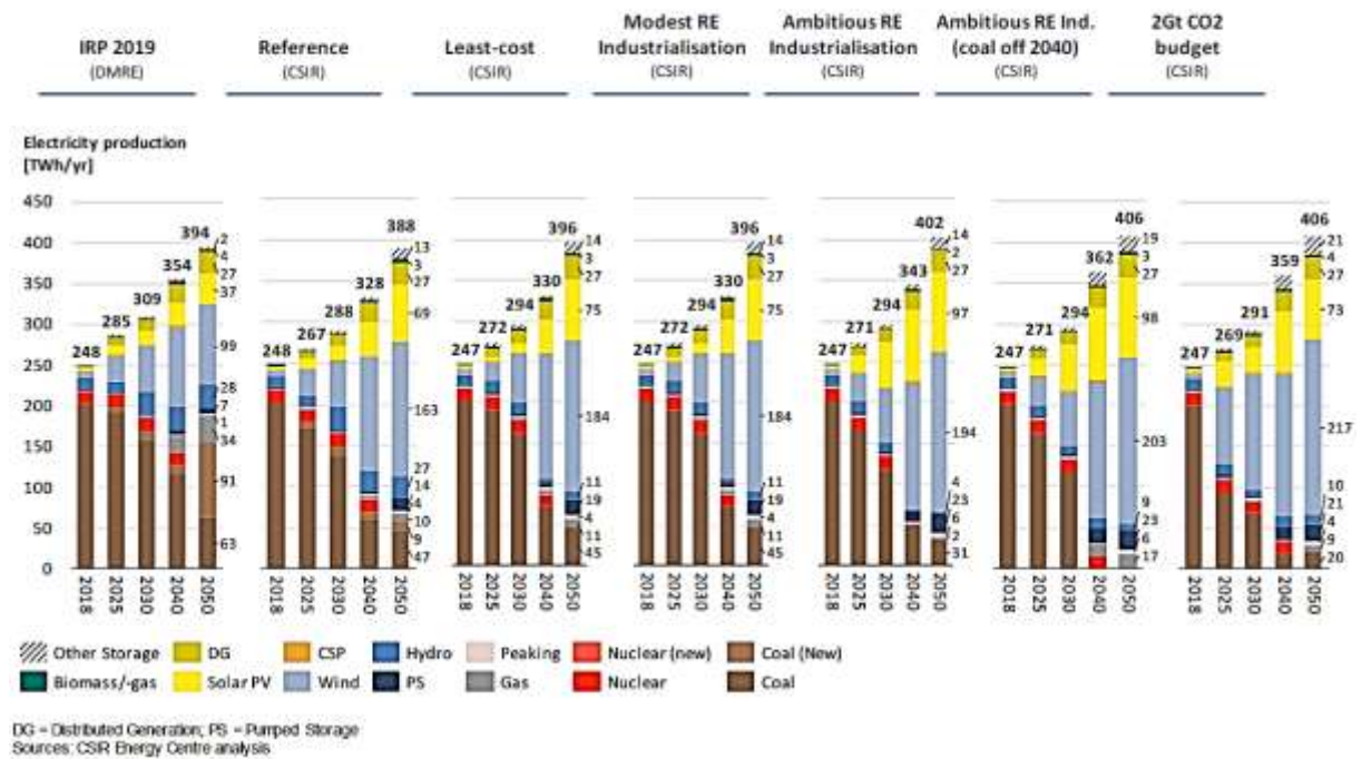
FIGURE 18: ELECTRICITY PRODUCTION BY SOURCE (TWH/YEAR)
